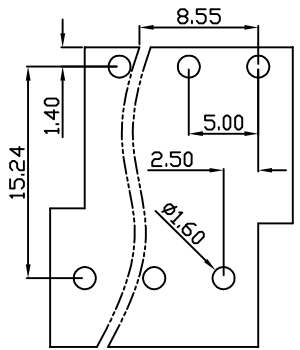
PCB Layout
