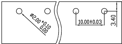
PCB Layout
